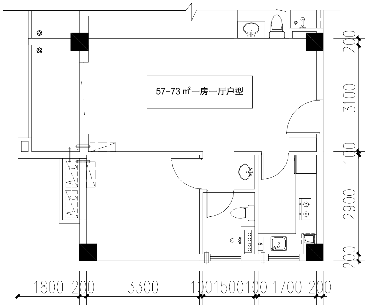
B 户型平面规划图 B FAMILY PLANNING DRAWINGS
