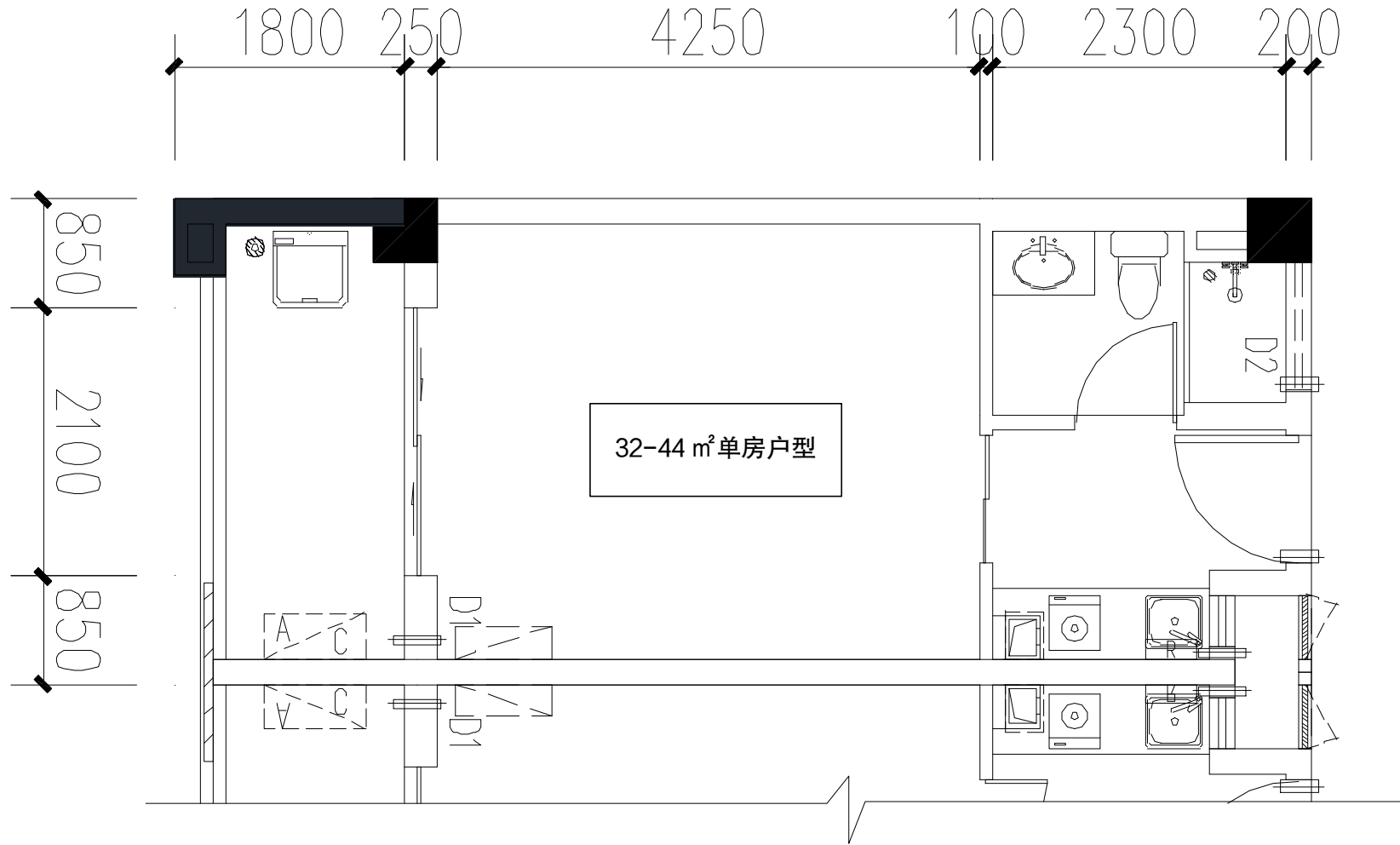
A 户型平面规划图 A FAMILY PLANNING DRAWINGS
